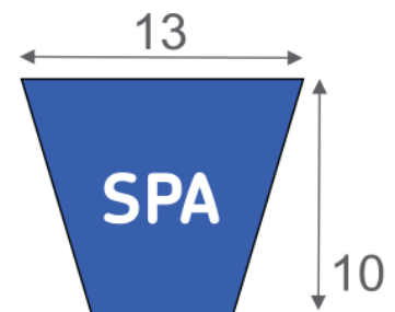
SKF Wrapped Classical V-Belt
